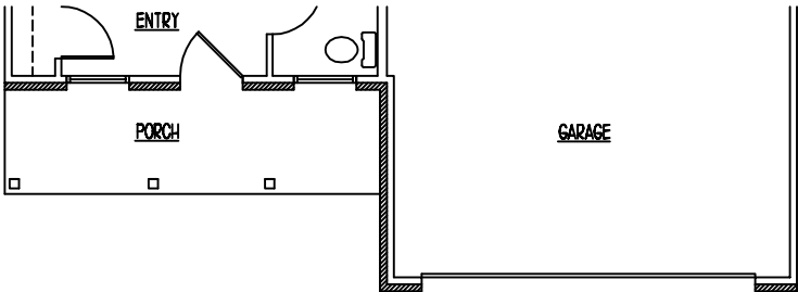
Option B Floor Plan - first floor added covered porch
